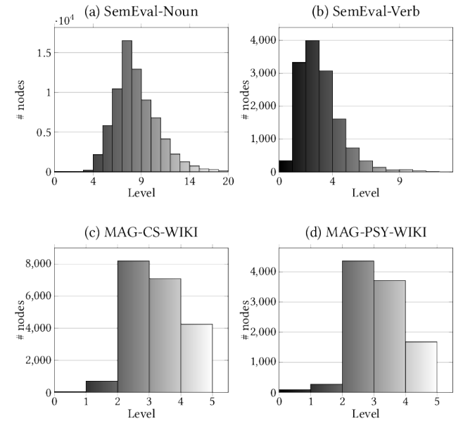
Figure 5: Distribution of nodes over the levels of the taxonomy in (a,b) SemEval and (c,d) MAG.
