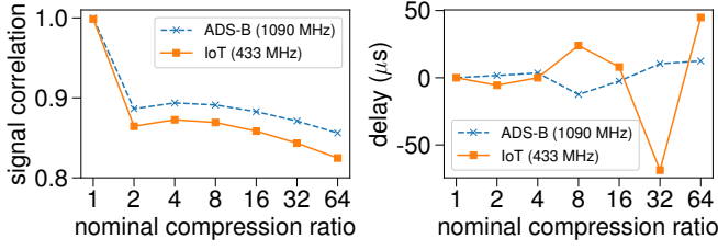
Fig. 12. Signal correlation and delay vs. nominal compression ratio for both IoT-433 and ADS-B. Up to compression factor of 4 the delay is acceptable for localization apps.
