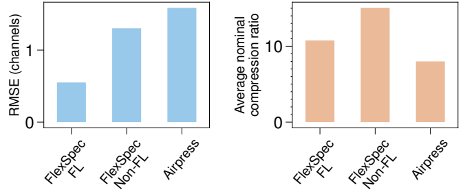
Fig. 14. RMSE of channels detected (left) and average nominal compression ratio for the different solutions evaluated over PSD data.
