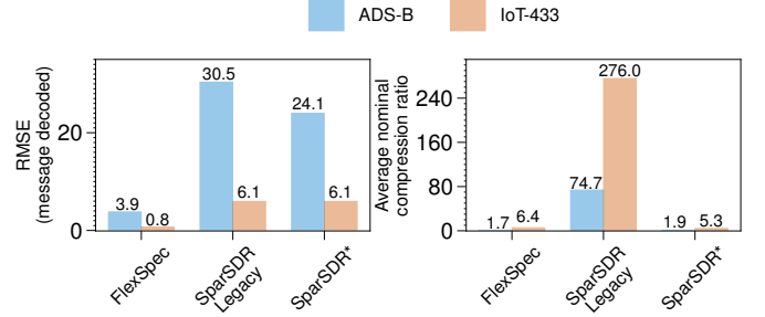
Fig. 18. Summary of IQ decoding performance and compression ratio using FlexSpec and SparSDR.
