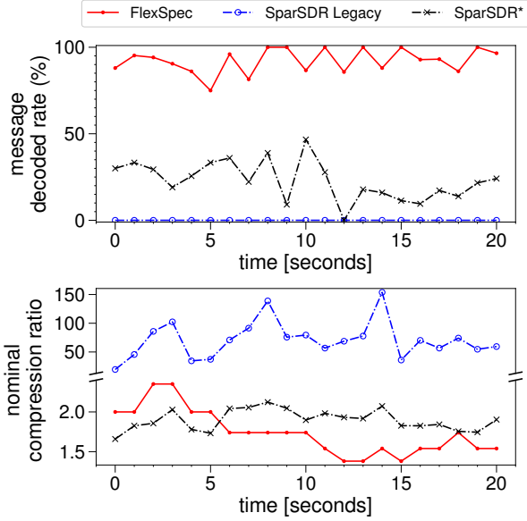
Fig. 16. ADS-B messages decoded and compression ratio used for FlexSpec and SparSDR.
