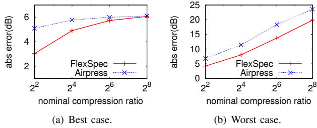
Fig. 8. 99th percentile reconstruction error as a function of nominal compression ratio. FlexSpec outperforms Airpress by up to 5 dB in both the best and the worst cases.
