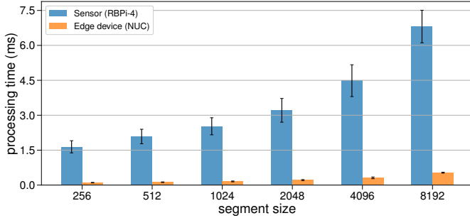
Fig. 19. FlexSpec compress/decompress latency performance in sensor (RBPi-4) and edge device (Intel NUC).
