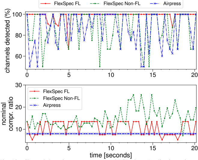
Fig. 13. Channel detection over compressed PSD data. Application-oriented compression ratio adaptation with Feedback Loop performs better than generic approaches.
