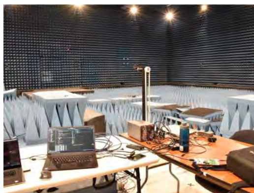
Experimental set-up in the lab in order to take over drones in a controlled environment via GPS spoofing.
